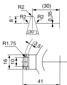
DETAIL OF SPRING PLATE
