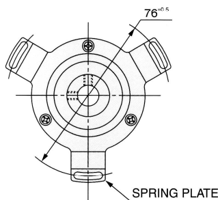
DETAIL OF SPRING PLATE
