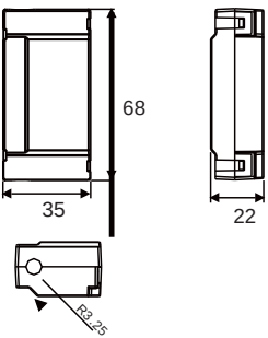
Single Battery Box ASD-MDBT0100
